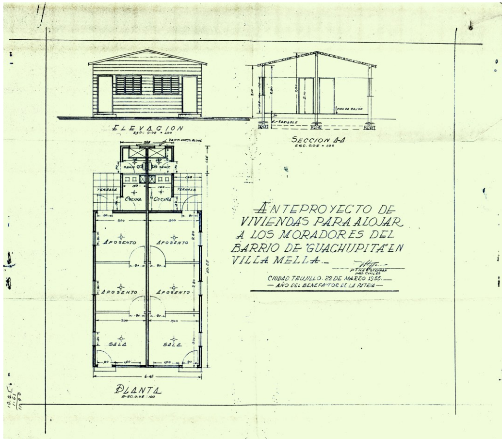
FIGURE 4. Preliminary housing project in Villa Mella (north of Santo Domingo) for the relocation of the population near the Ozama river. Source: AGN, Fondo Presidencial, Documentación posterior a 1953, código 10492-2, caja 3107801, sin legajo.
